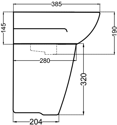
SIDE VIEW WITH PEDESTAL
